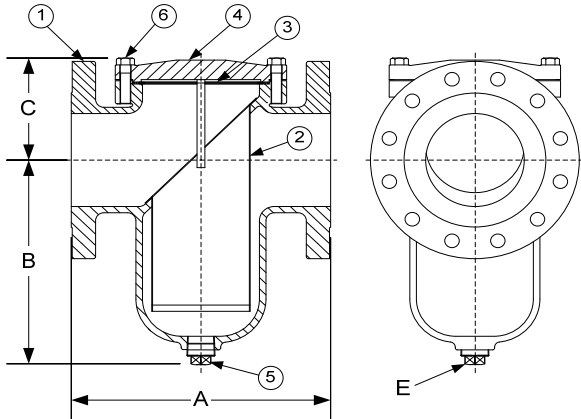
Style SSGFV - Bolted Cover (Shown Above) Available in 150 lb. and 300 lb. Class
